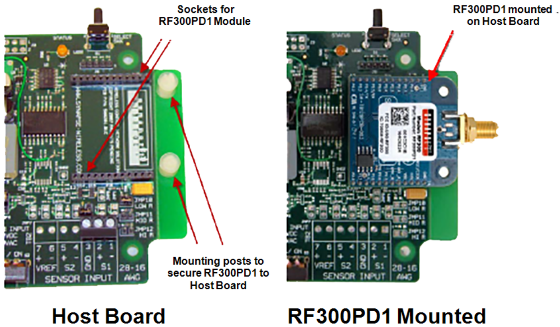
Figure 1.2: RF300PD1 Mounted To Host Board
